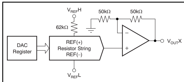
Figure 92. DAC8564 Architecture
